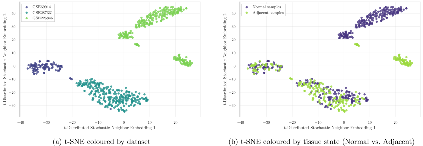
Figure 20: Two views of the t-SNE embedding computed on the 326k CpGs shared across GSE69914, GSE225845, and GSE287331.
